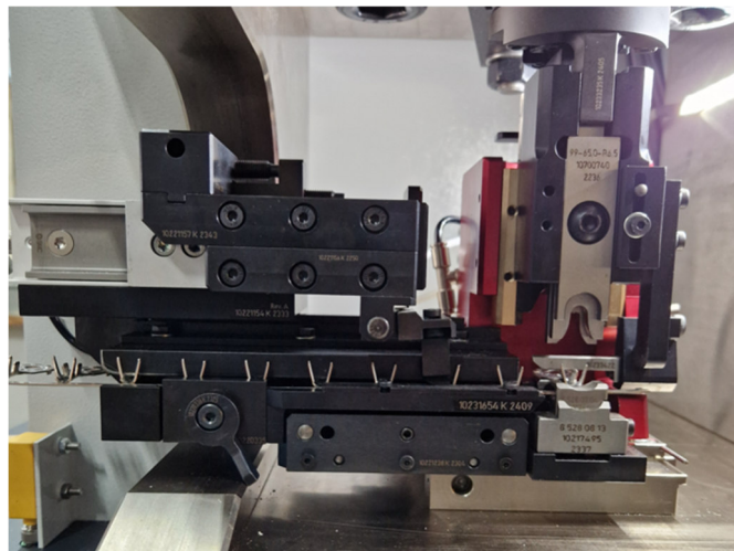
Crimping tool JG for JTHP
